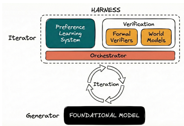
Figure 4: The Harness Architecture
