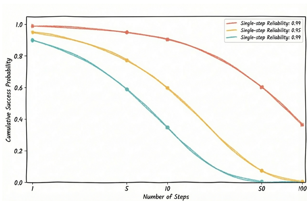
Figure 2: Degredation of Multi-Step LLM Reasoning Reliability
